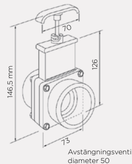
Gate valve diameter 50
