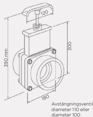
Gate valve diameter 110
